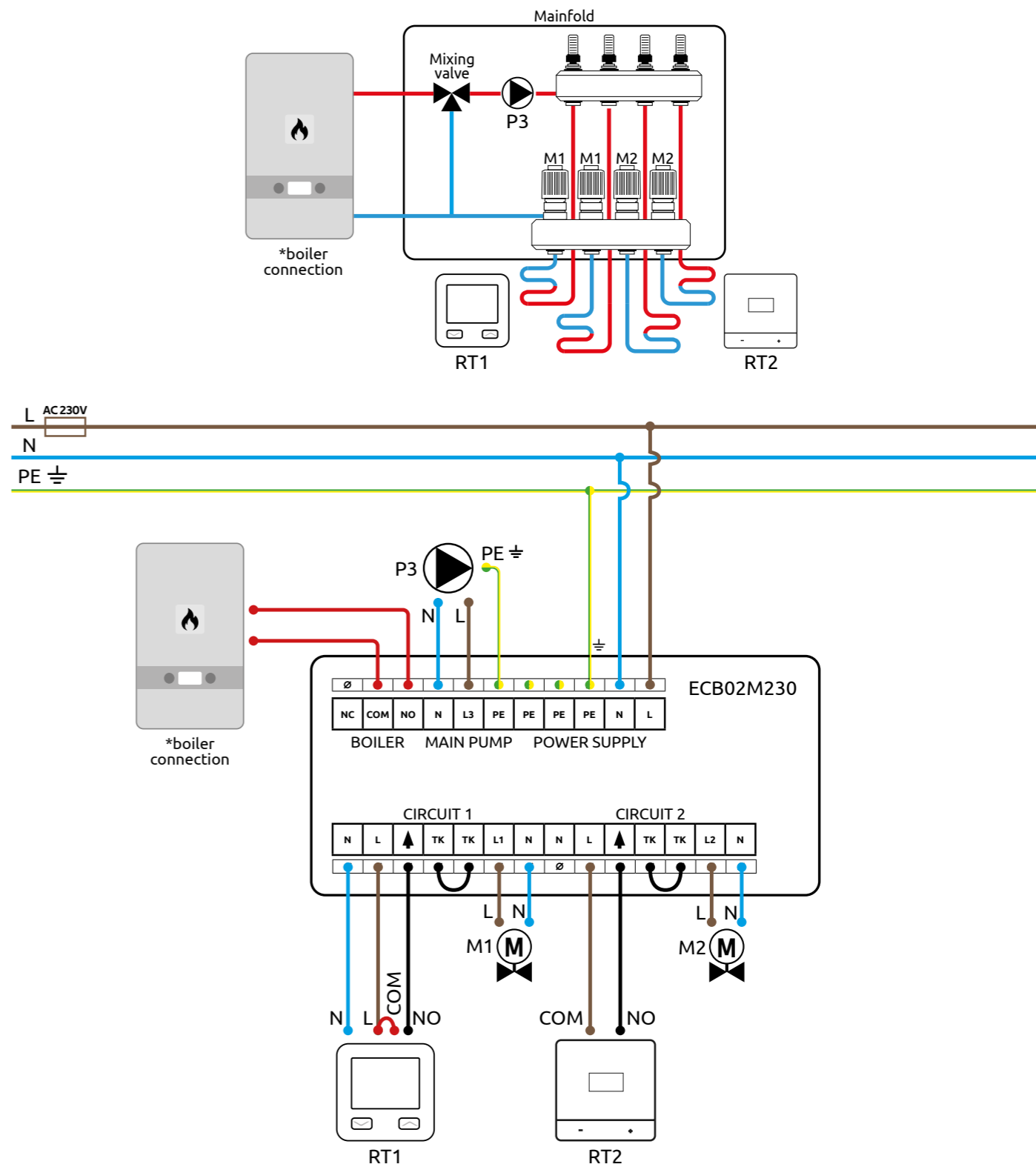
b) - Connection of 2 underfloor heating zones
