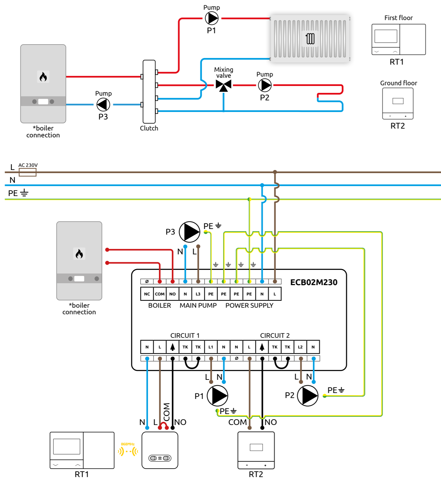
a) - Connection of 2 heating circuits
