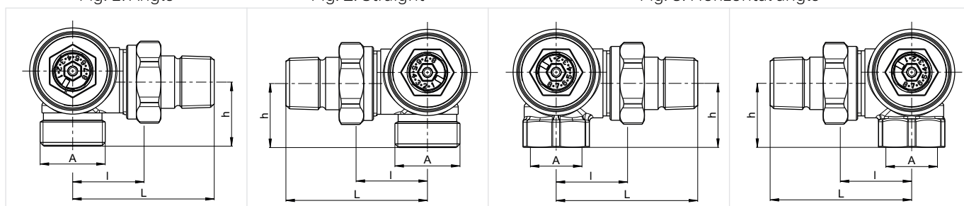
Fig 4. Double angle left, G 3/4"
